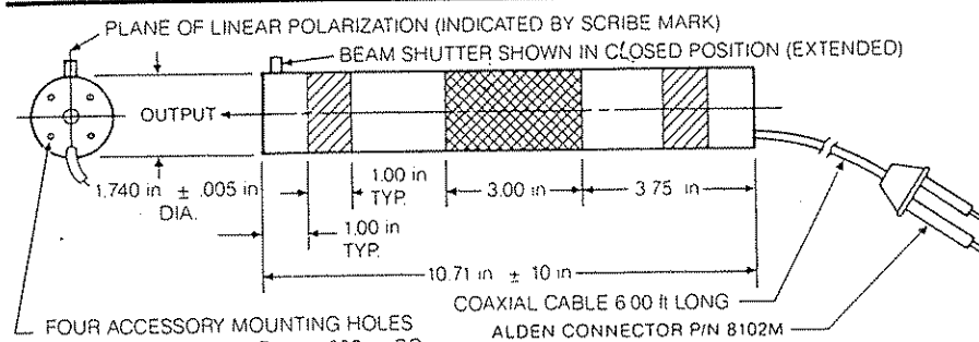
1 and 2 mW MODELS WITH H.V. CABLE AND CONNECTOR AND BEAM SHUTTER
