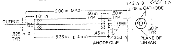
INTERNAL MIRROR PLASMA TUBE
