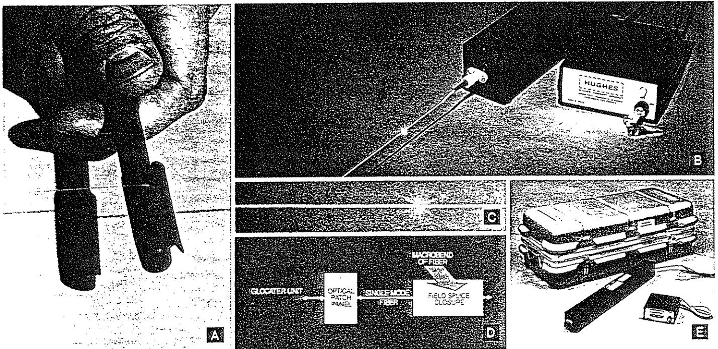
Easily induced macrobend (12 mm is ideal) produces visible glow (A). Breaks show clearly (B) and (C). Connects directly to patch panel (D). Comes complete with carrying case (E).
