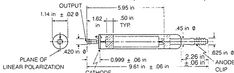
INTERNAL MIRROR PLASMA TUBE
