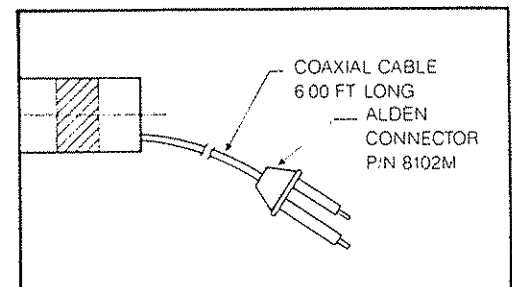
WITH H.V. CONNECTOR (H-C and H-PC MODELS) (All other dimension same as H and H-P models)
