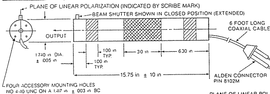
4 & 5 mW MODELS WITH HIGH VOLTAGE CONNECTOR AND BEAM SHUTTER
