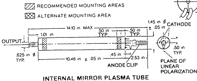
INTERNAL MIRROR PLASMA TUBE
