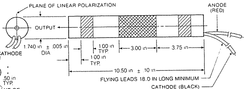
1 and 2 mW MODELS WITH FLYING LEADS
